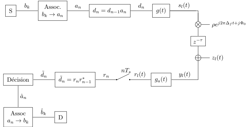
FIGURE 1 – Architecture bande de base sans synchronisation
